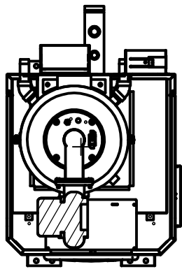
SECTION A-A SCALE 0.1
